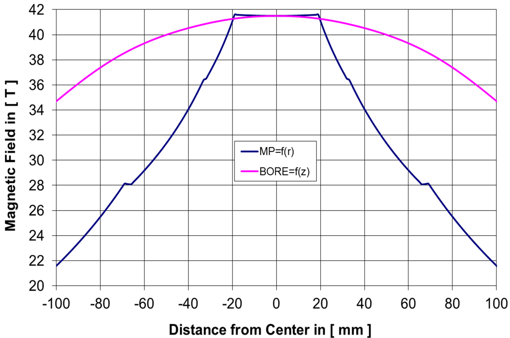
Magnetic Field Profiles along Bore & Mid-plane @ FULL current
